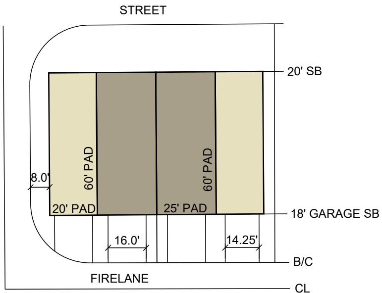
TYPICAL LOT
